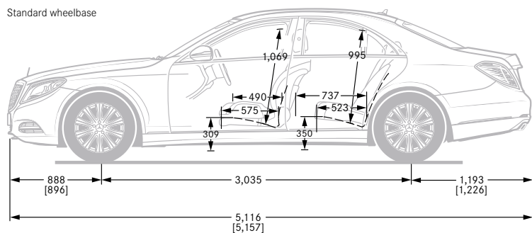
Standard wheelbase
