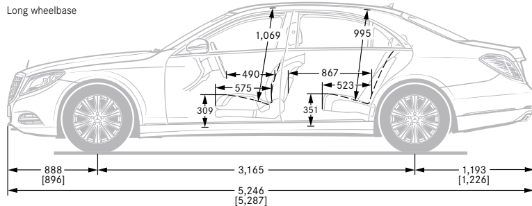
Long wheelbase
